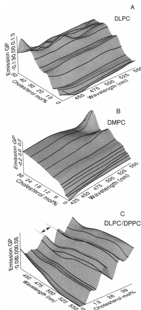
FIGURE 2 Surface representation of the variation of Laurdan emission GP spectra obtained at 25°C as a function cholesterol concentration in phospholipid vesicles composed of DLPC (A), DMPC (B), and an equimolar mixture of DLPC and DPPC (C). The spectra and the surface have been obtained as reported for Fig. 1. The emission GP spectra have been calculated using Eq. 3. Arrows (C) represent the cholesterol region that has been expanded by 1 mol % cholesterol increase (shown in Fig. 7 B, below).
